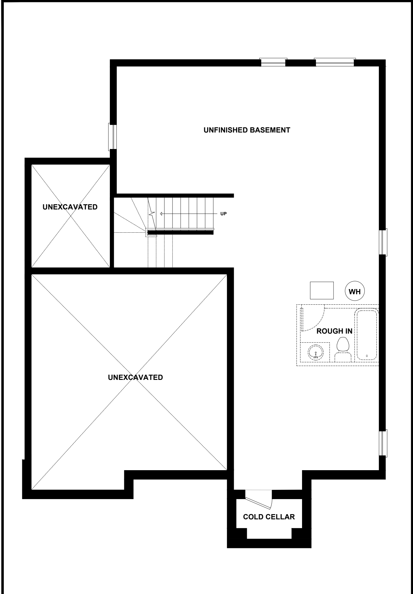
BASEMENT PLAN
