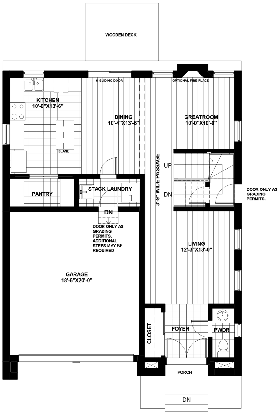
GROUND FLOOR : 943 sq.ft.
