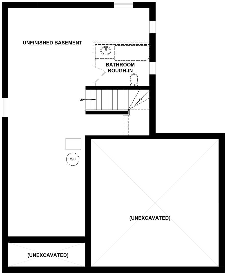
BASEMENT FLOOR
