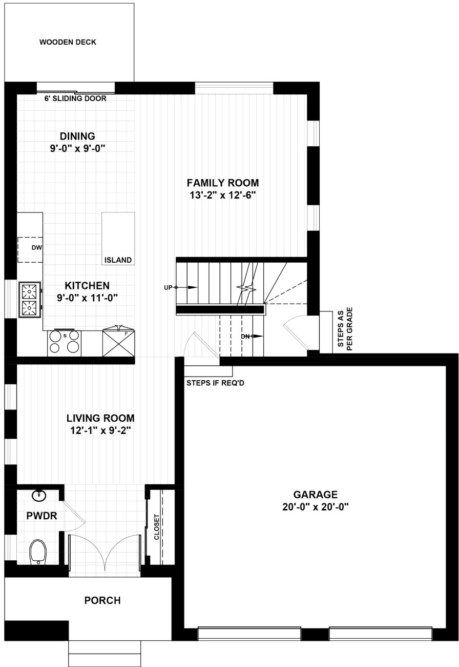
GROUND FLOOR : 737 sq.ft.
