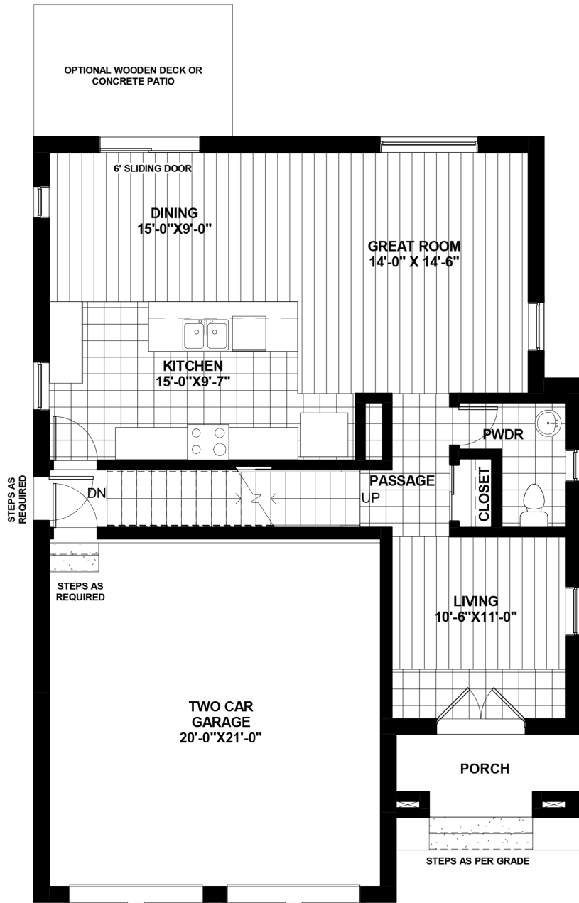
GROUND FLOOR ELEVATION A : 900 sq.ft.
