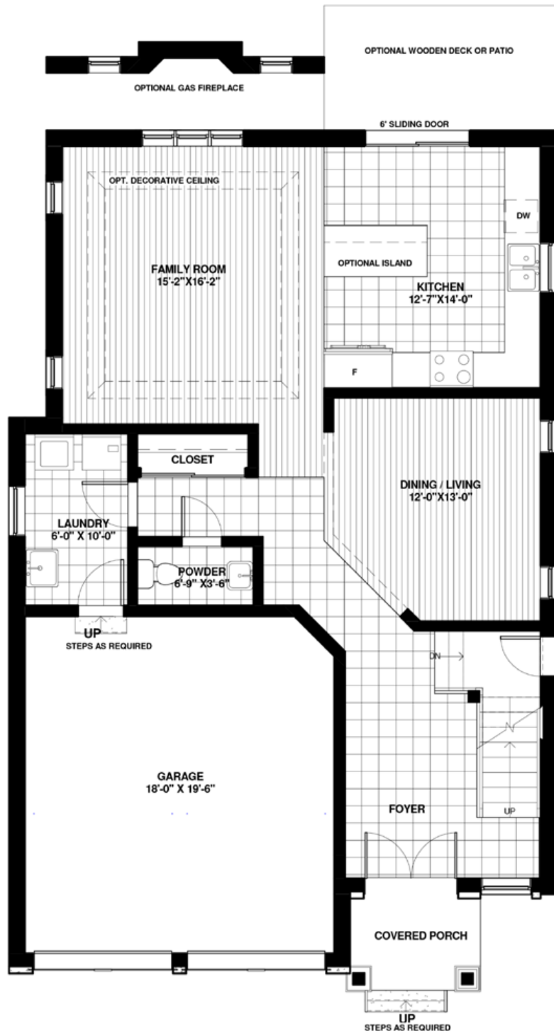
GROUND FLOOR : 1068 sq.ft.
